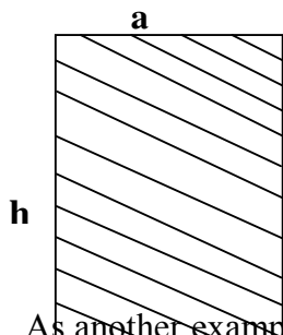
As another example of a max-min problem, let us determine the length and the width of a sandbox whose height is 1 ft and which hold 25 cub ft of sand, in other that the minimum amount of wood will be used in constructing it.
